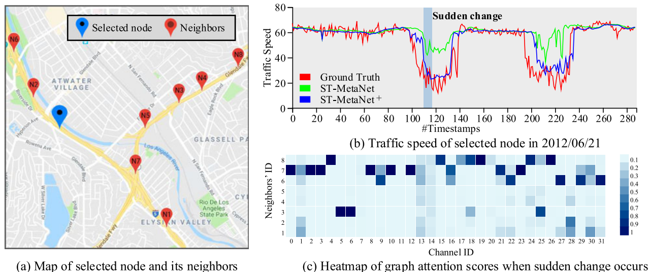
Fig. 15. Case study for a sudden change of traffic speed on METR-LA dataset.
