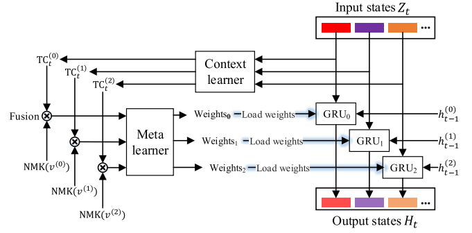
Fig. 7. Structure of Meta-GRU + .
