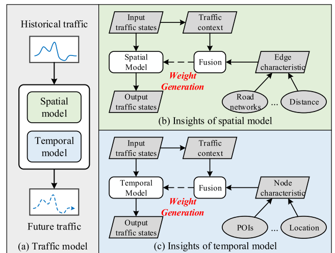
Fig. 4. Insights of our framework.
