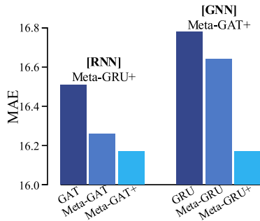
Fig. 8. Ablation studies on taxi flow prediction.
