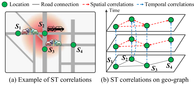
Fig. 1. Complex composition of ST correlations.
