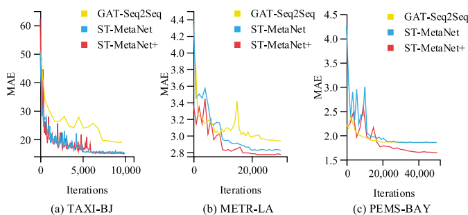
Fig. 13. Framework convergence on validation datasets.
