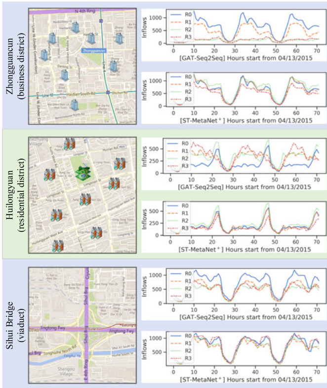
Fig. 14. The inflows of the representative grids. The left maps show the selected grids with special functions, i.e., business district, residential district, and viaduct. The right charts show the inflow trends of the selected grids R_0 and its k -nearest neighbors R_k ( k > 0 ) in the embedding space produced by GAT-Seq2Seq and ST-MetaNet + .
