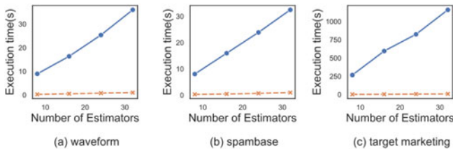
Fig. 6. Prediction time versus number of estimators.
