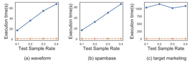
Fig. 8. Prediction time versus test sample size.
