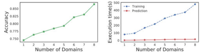
Fig. 4. Accy. & Exec. time versus # of domains.
