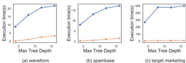
Fig. 7. Prediction time versus max depth.
