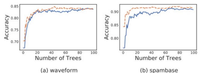
Fig. 5. Convergence.
