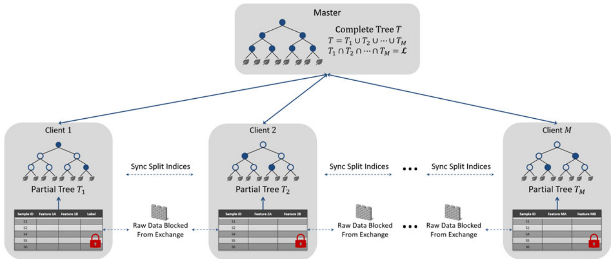
Fig. 2. Federated forest.
