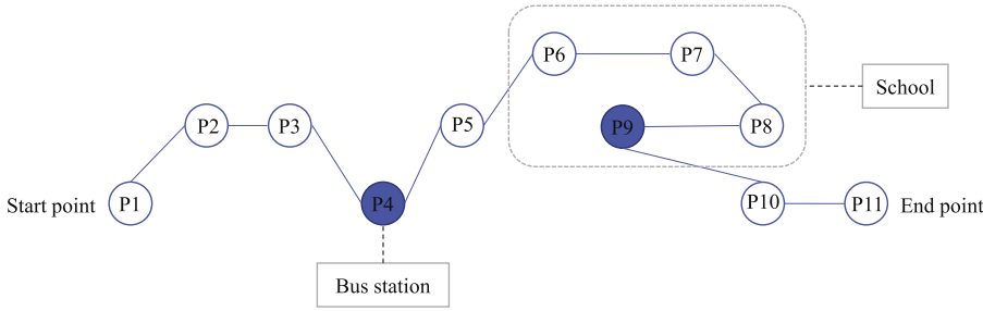
Fig. 2. Stay points and regions in trajectories.
