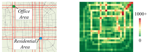
Figure 2: Regions in Beijing: (a) Grid-based map segmentation; (b) inflows in every region of Beijing
